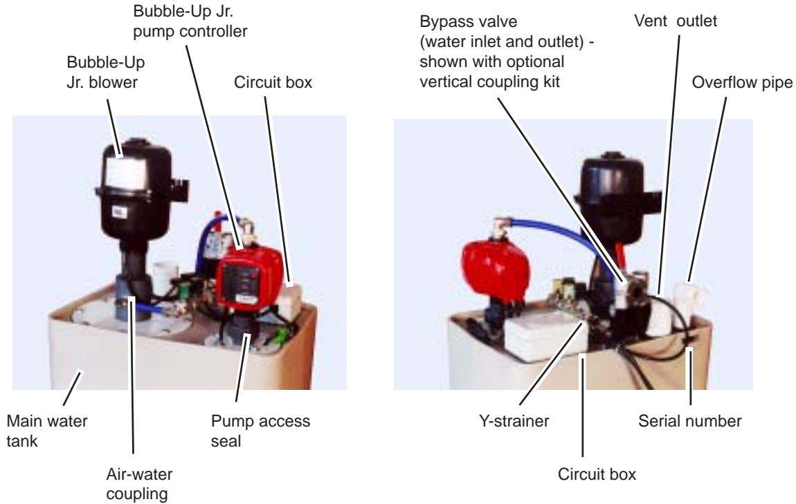
Fig. 2 Installation Points
