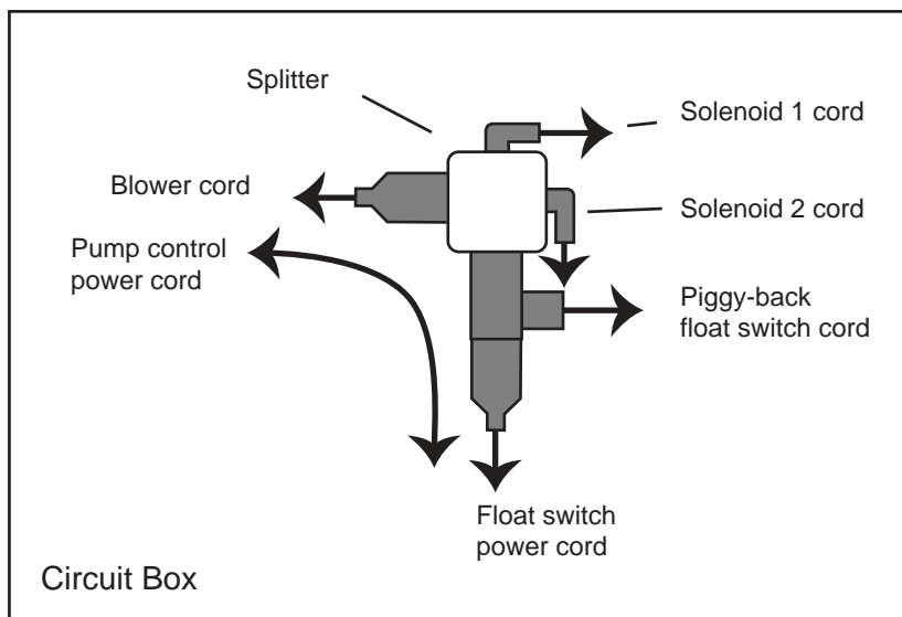
Fig. 3 Wiring Connections
